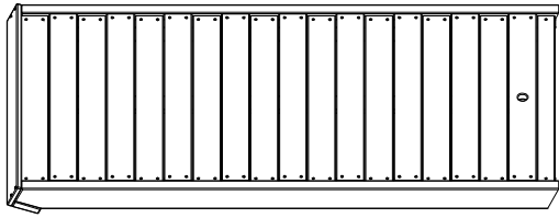
ROPE WALL ASSEMBLY
