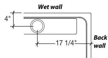
Drain Location Detail
