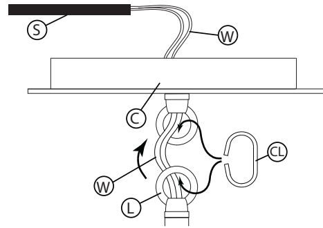
DRAWING 2 - MOUNTING
