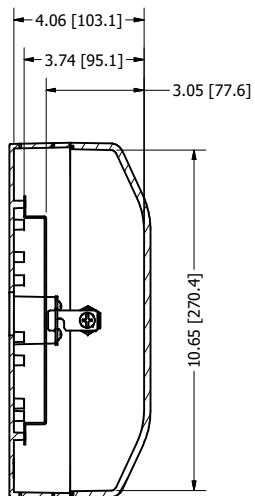
SECTION A-A SCALE 1 / 3
