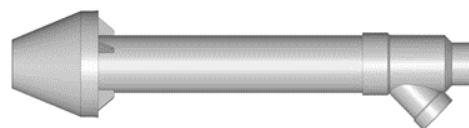
Sample DiversiTech 2 in. and 3 in. Concentric Vent Termination
