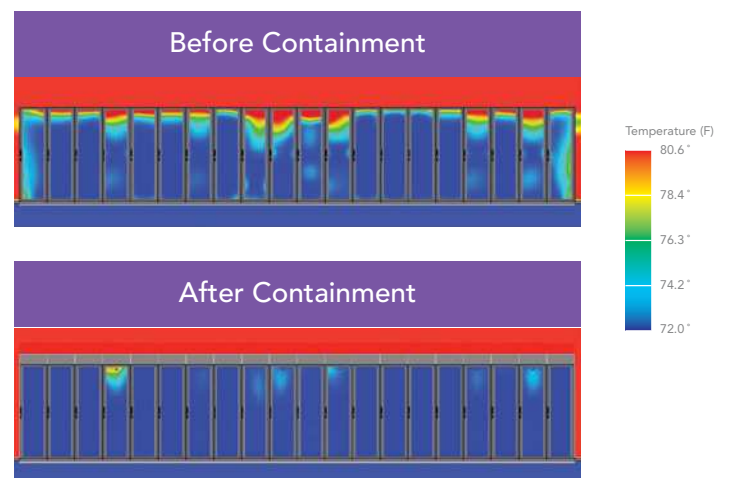
CFD analysis shows evenly distributed temperatures and reduced hot spots after the installation of Rack Top Angle Baffles in the cold aisle.
