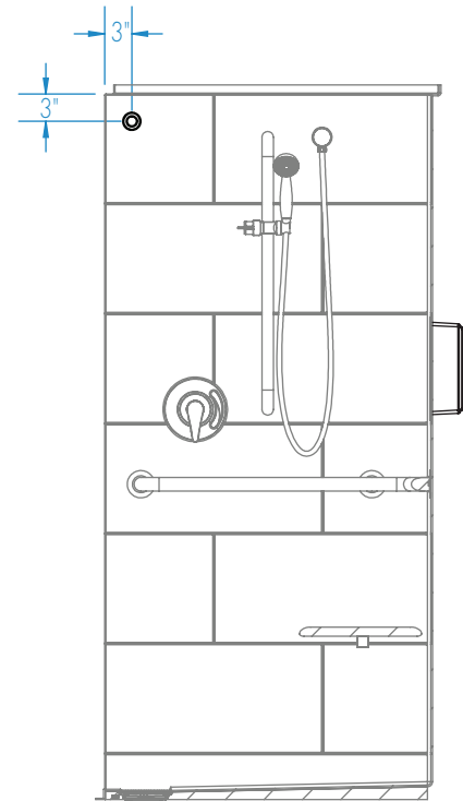
SECTION C-C
