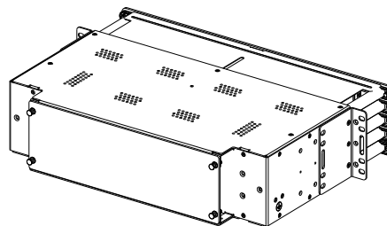
96 Port Rear View with Rear Protection
