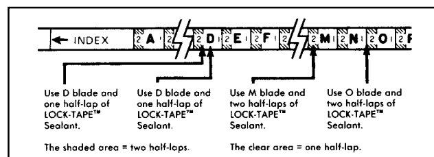
FIGURE 5 – SKETCH OF MEASURE TAPE
