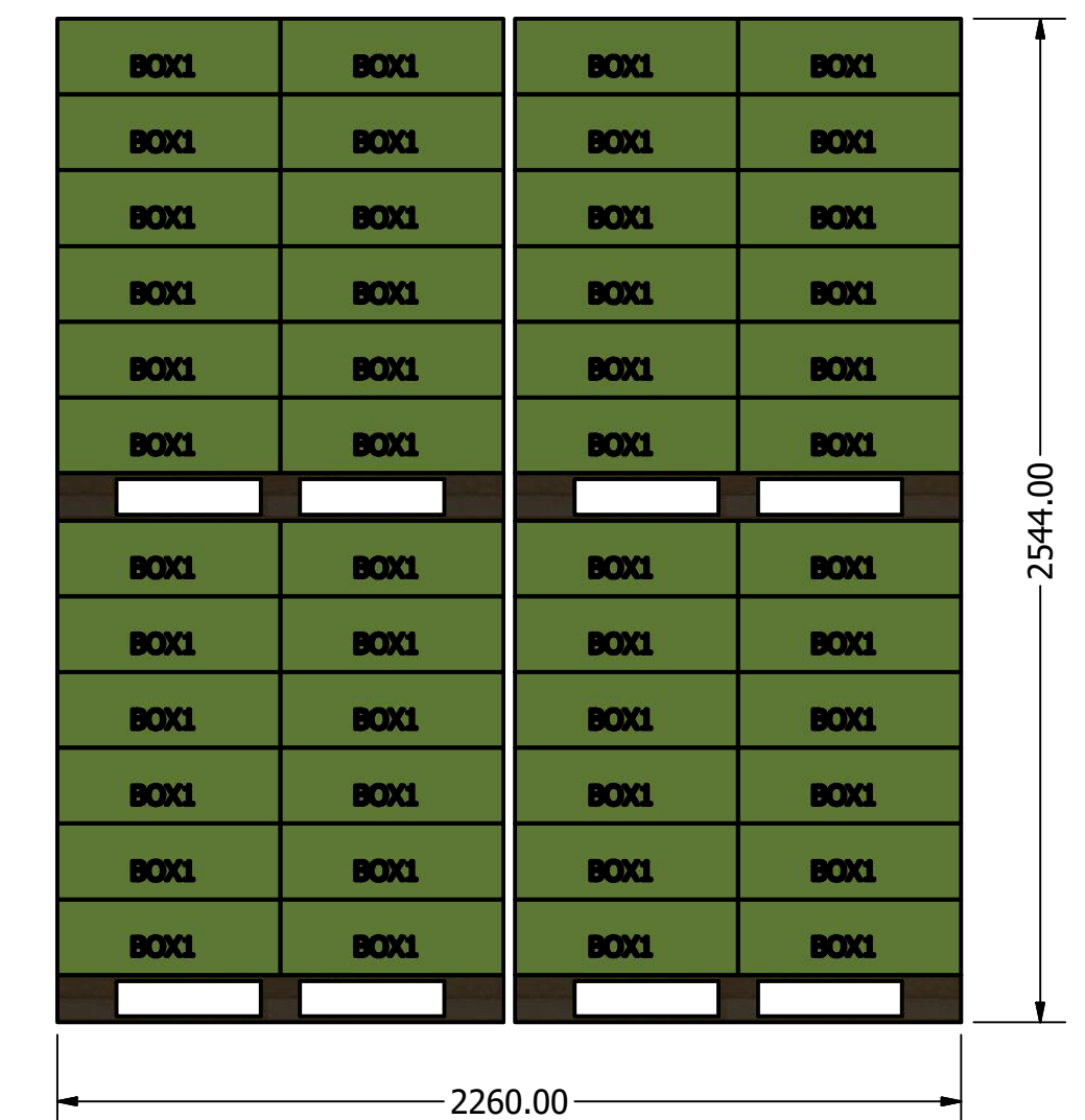
End View
