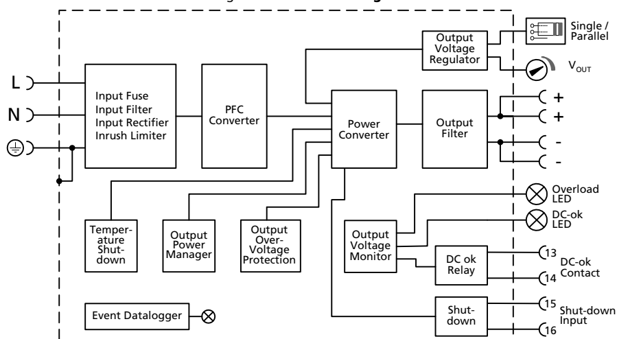
Fig. 14-1 Functional diagram
