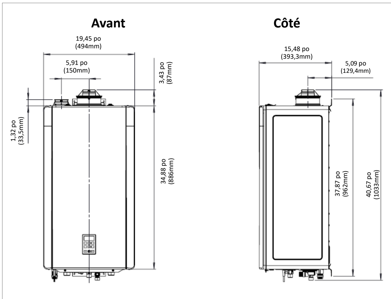
Figure 5: Dimensions
