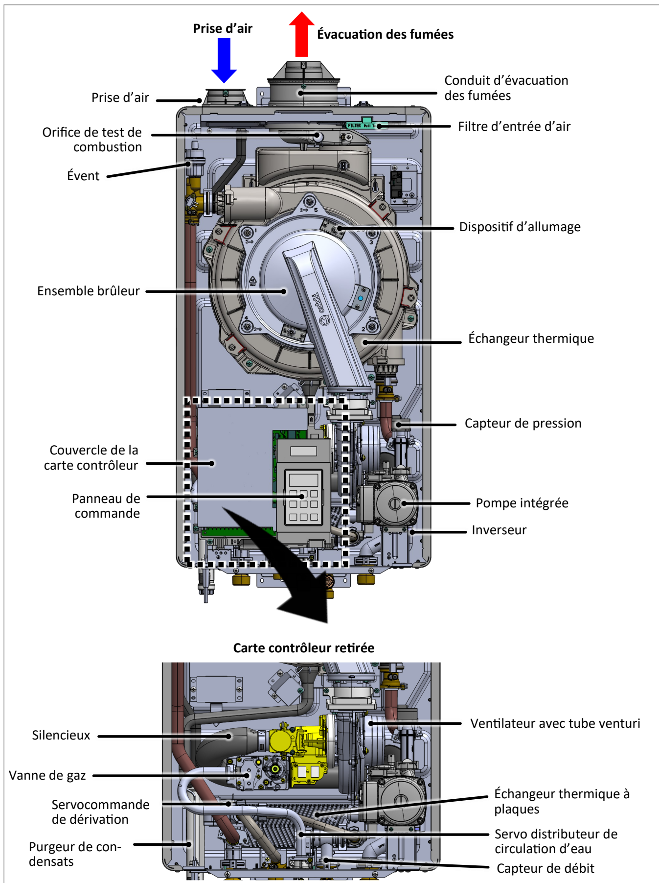
Figure 4: Composants
