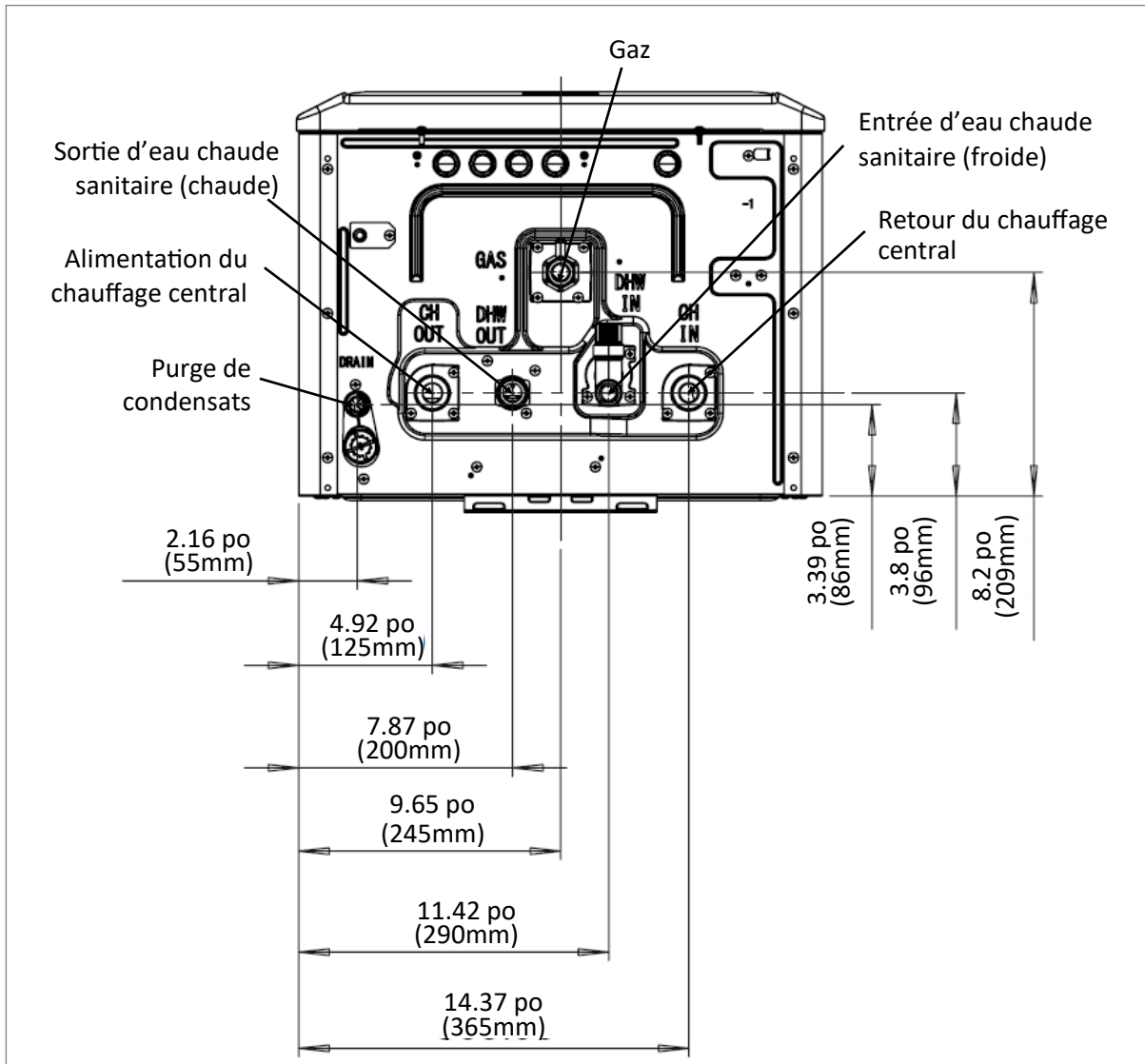
Figure 6: Raccords d'alimentation
