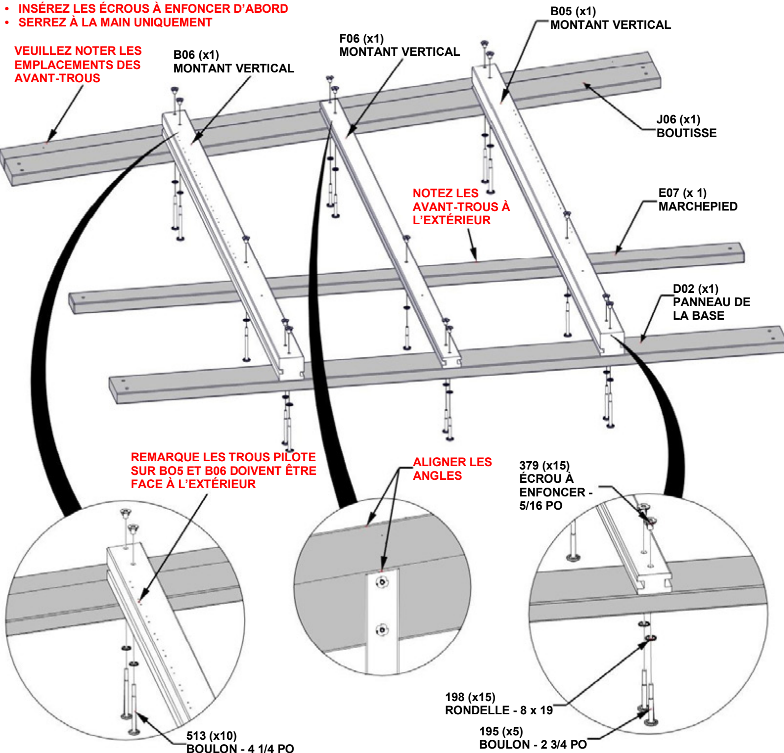
B06 MONTANT VERTICAL - W4L18687 (x1) 3 po x 3 po x 78 3/4 po (76x76x2000)
