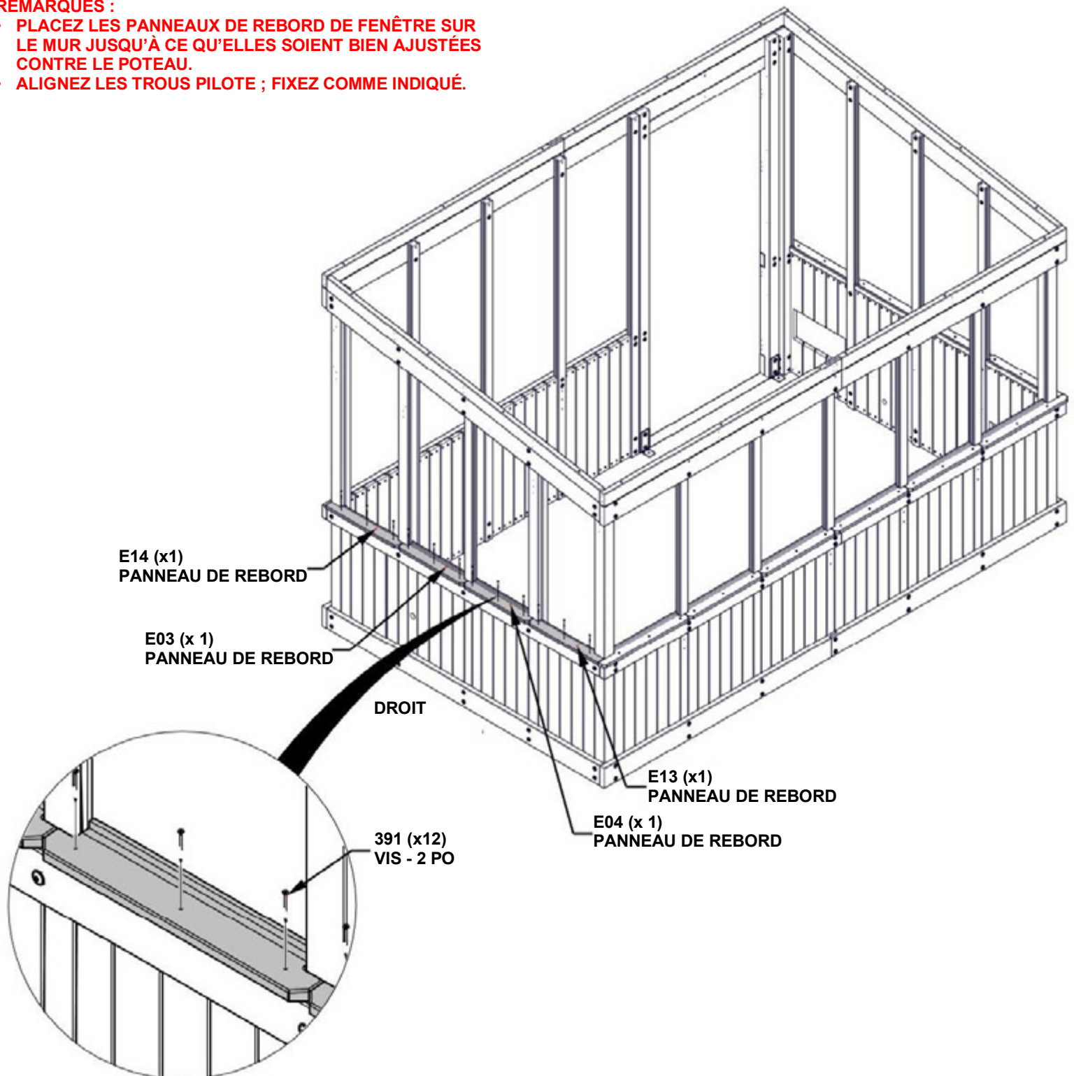
E03 PANNEAU DE REBORD - W4L18695 (x1) 1 7/16 po x 3 3/8 po x 19 15/16 po (36x86x507)
