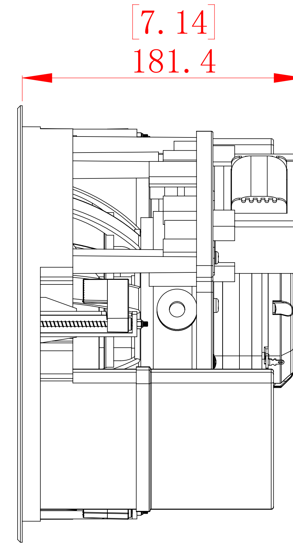
MOUNTING DEPTH
