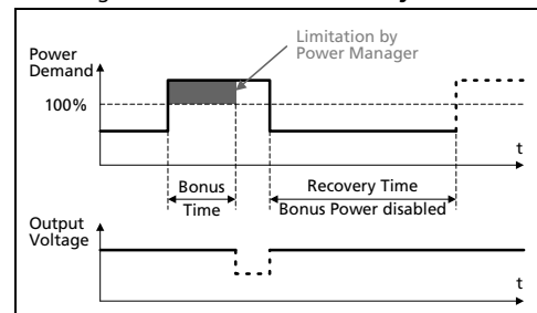
Fig. 6-4 BonusPower® recovery time
