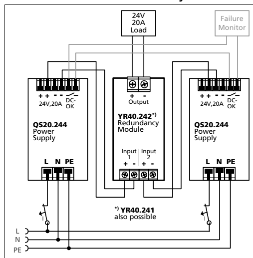
Fig. 21-1 Typical 1+1 Redundant configuration for 20A with a dual redundancy module
