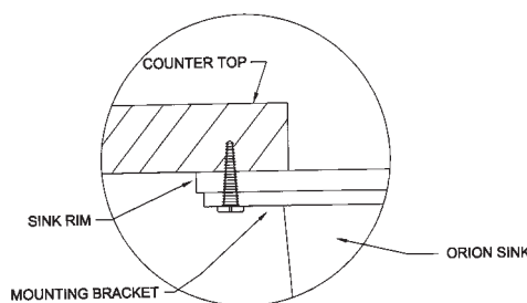
Under counter installation detail
