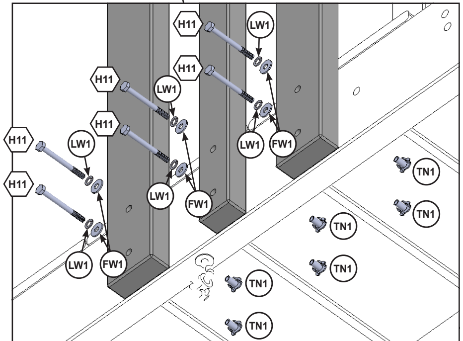
Underneath View
