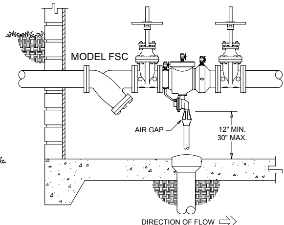
INDOOR INSTALLATION
