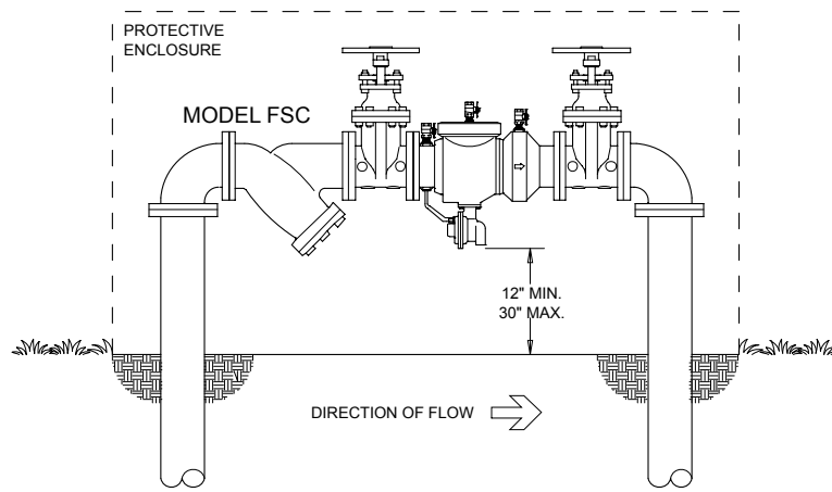
OUTDOOR INSTALLATION
