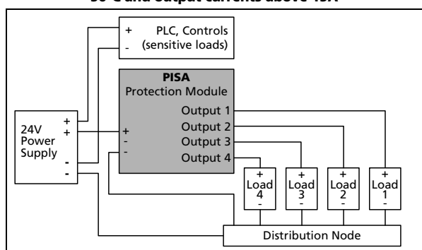
Fig. 3-2 Wiring scheme for ambient temperatures above 50°C and output currents above 15A
