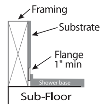
Flange Details: (U.S.)
