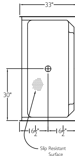
TOP VIEW
