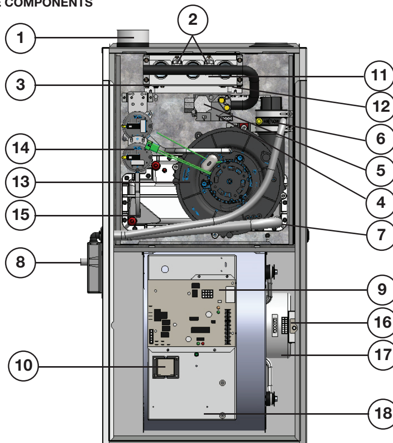
FIGURE 34 - FURNACE COMPONENTS
