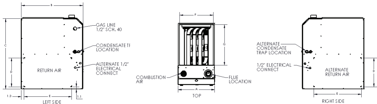
FIGURE 1 - FURNACE DIMENSIONS AND CLEARANCE TO COMBUSTIBLES
