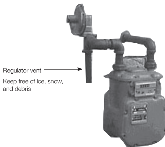
FIGURE 2 - GAS REGULATOR VENT
