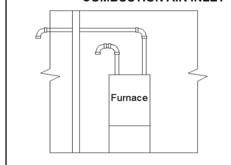
FIGURE 7 - NON-DIRECT COMBUSTION AIR INLET
