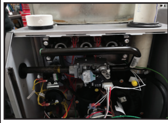
FIGURE 24 - INSHOT BURNER ASSEMBLY
