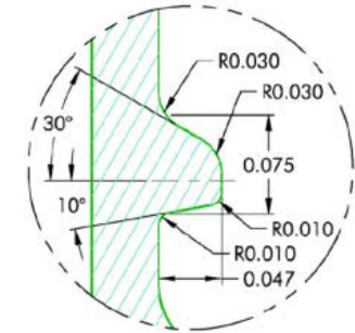
GLASS THREAD DETAIL SCALE 10 : 1
