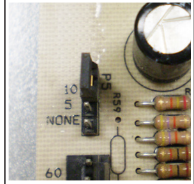
FIGURE 32 - JUMPER P5
