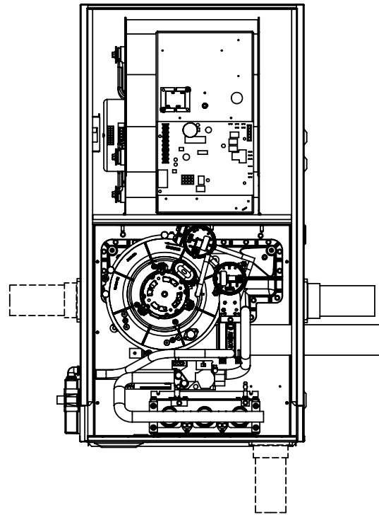
LEFT VENT INSTALLATION - RIGHT DRAIN (EXTERNAL)
