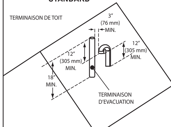
FIGURE 11 - CONFIGURATION D'ÉVACUATION VERTICALE STANDARD
