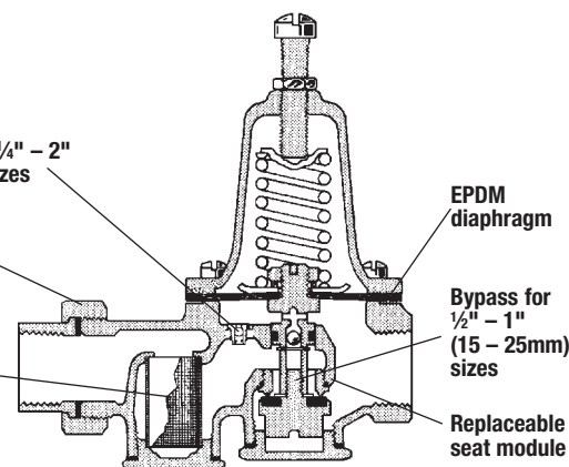
Integral stainless steel strainer
