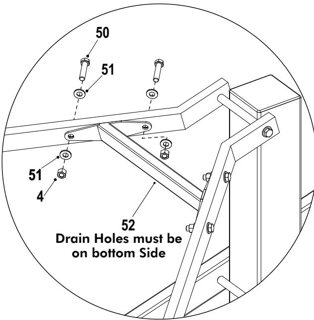
Detail C
