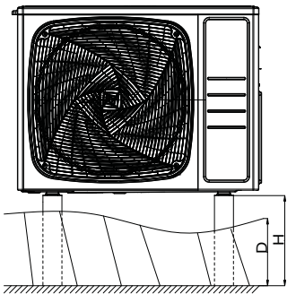
Correct Installation
