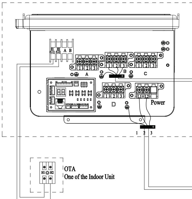
Outdoor unit
