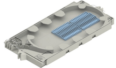
COYOTE Legacy Long Deep Profile Splice Tray Kit for Ribbon/Mass Fusion Splices (144 Splice CT.) Catalog Number: 80805515
