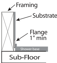
Flange Details: (U.S.)
