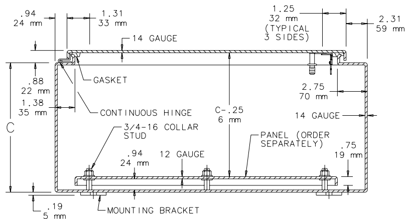
SECTION X-X
