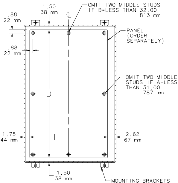
SECTION Y-Y
