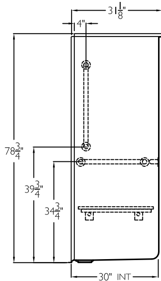
CROSS SECTION OF SHOWER BASE
