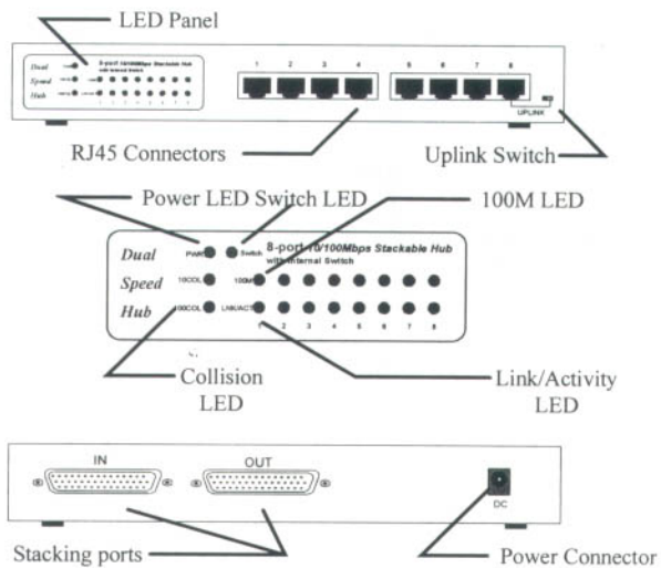
Figure 4-1 Panel description (cont.)
