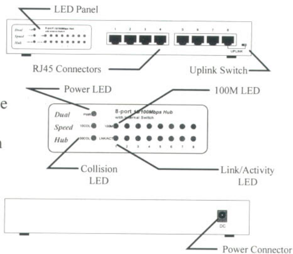
Figure 4-1 Panel description
