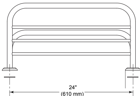
Mounting Specification
