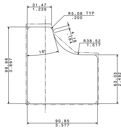
LABEL DETAIL (RECOMMENDED) Scale: 1:1
