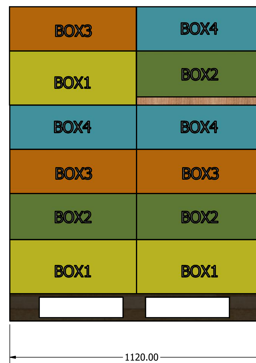
End View
