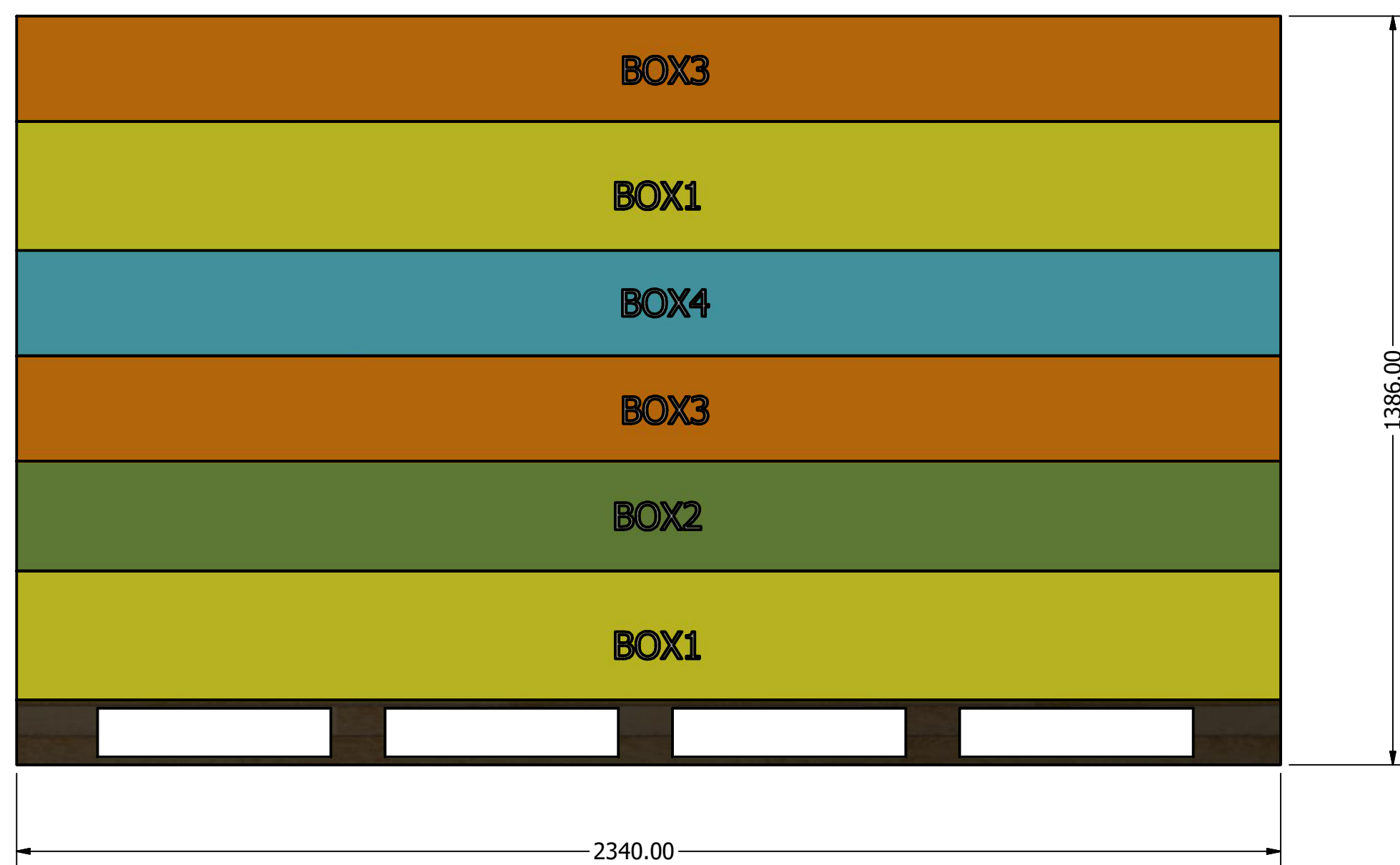
Side View
