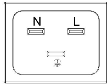
IEC60320 C20
