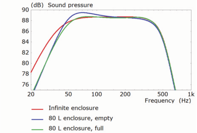
Figure 18. Effect of the ‘reasonable’ enclosure volume on the Ci250RRM-THX woofer frequency response
