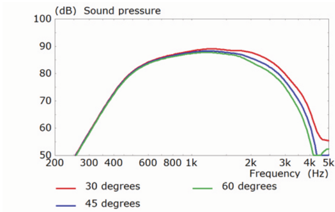
Figure 9. Midrange frequency response associated with Figure 8 (FEA modelled)
