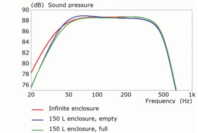
Figure 17. Effect of the ‘ideal’ enclosure volume on the Ci250RRM-THX woofer frequency response
