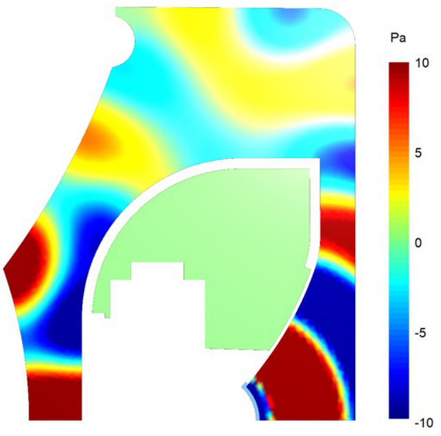
Figure 14. Tweeter pressure distribution at 8kHz associated with Figure 1
