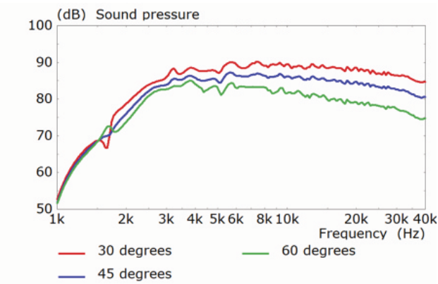
Figure 10. Tweeter response associated with Figure 1 (FEA modelled)
