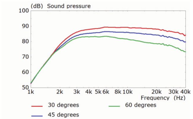
Figure 11. Tweeter response associated with Figure 8 (FEA modelled)
