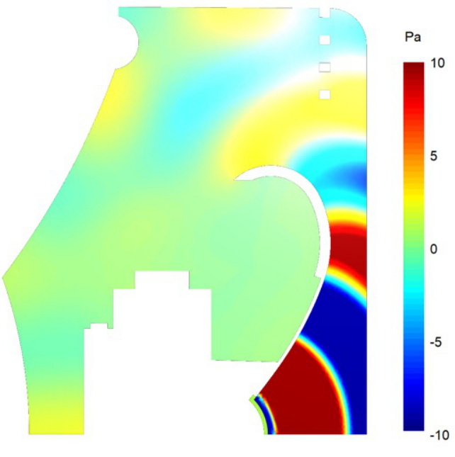
Figure 15. Tweeter pressure distribution at 8kHz associated with Figure 8
