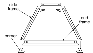
Frame construction for recessed panels
