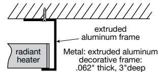
Frame construction for surface mount panels
