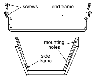
Frame construction for surface mount panels
