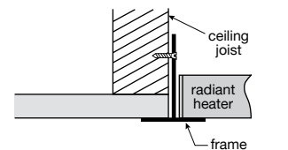
Frame construction for recessed panels
