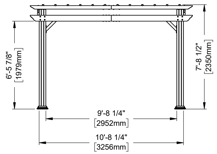
16' X 12' METAL PERGOLA FOOTPRINT
