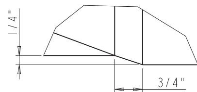
DETAIL A SCALE 2:5
