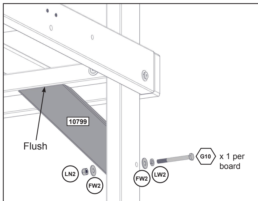
Underneath View
