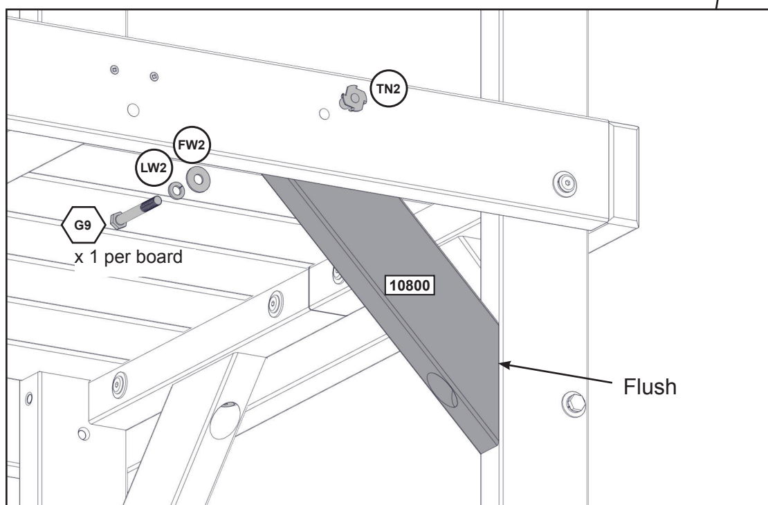
Underneath View
