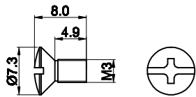
K4-6x8mm (M3x5mm)
