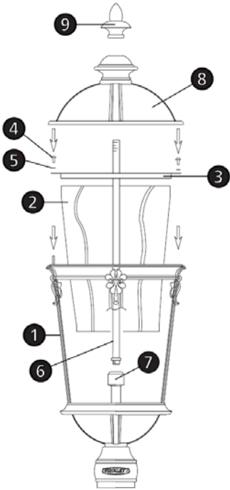
Drawing 2 – Fixture Mounting
