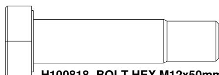
H100818 BOLT HEX M12x50mm WZ (x6) M12x 50mm
