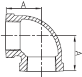
90 Elbow
