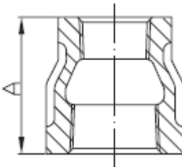
Reducing Coupling
