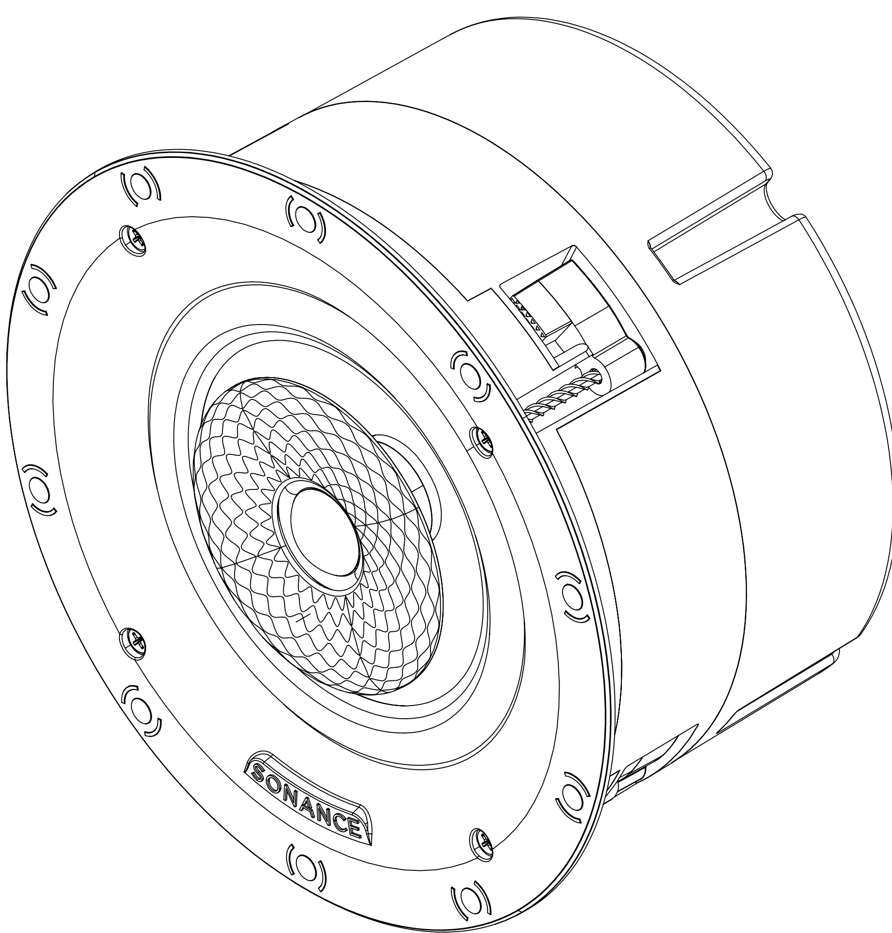
ISOMETRIC
