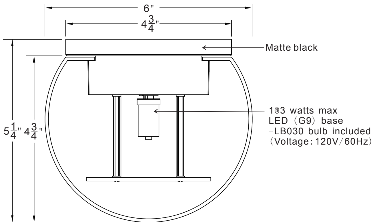
BOTTOM VIEW
