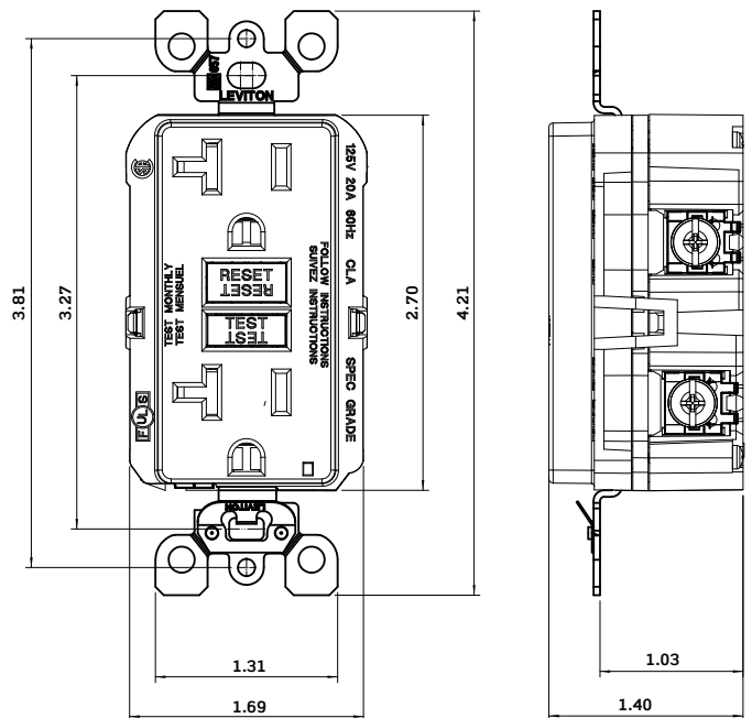
20A SmartlockPro® Self-Test GFCI
