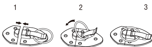
Outer buckle installation
