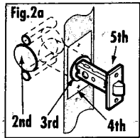
3 Hole Straddle-refer template (alternatively, drill 50/54mm hole through door face)
