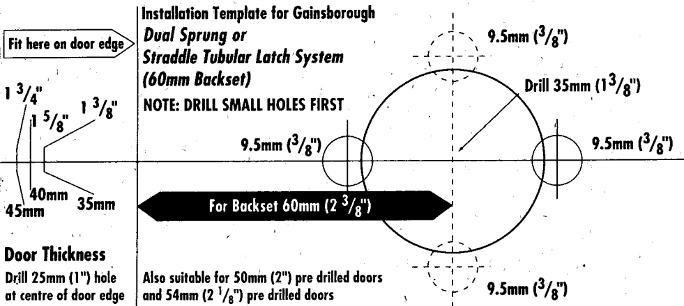
3 Hole Straddle-refer template (alternatively, drill 50/54mm hole through door face)
